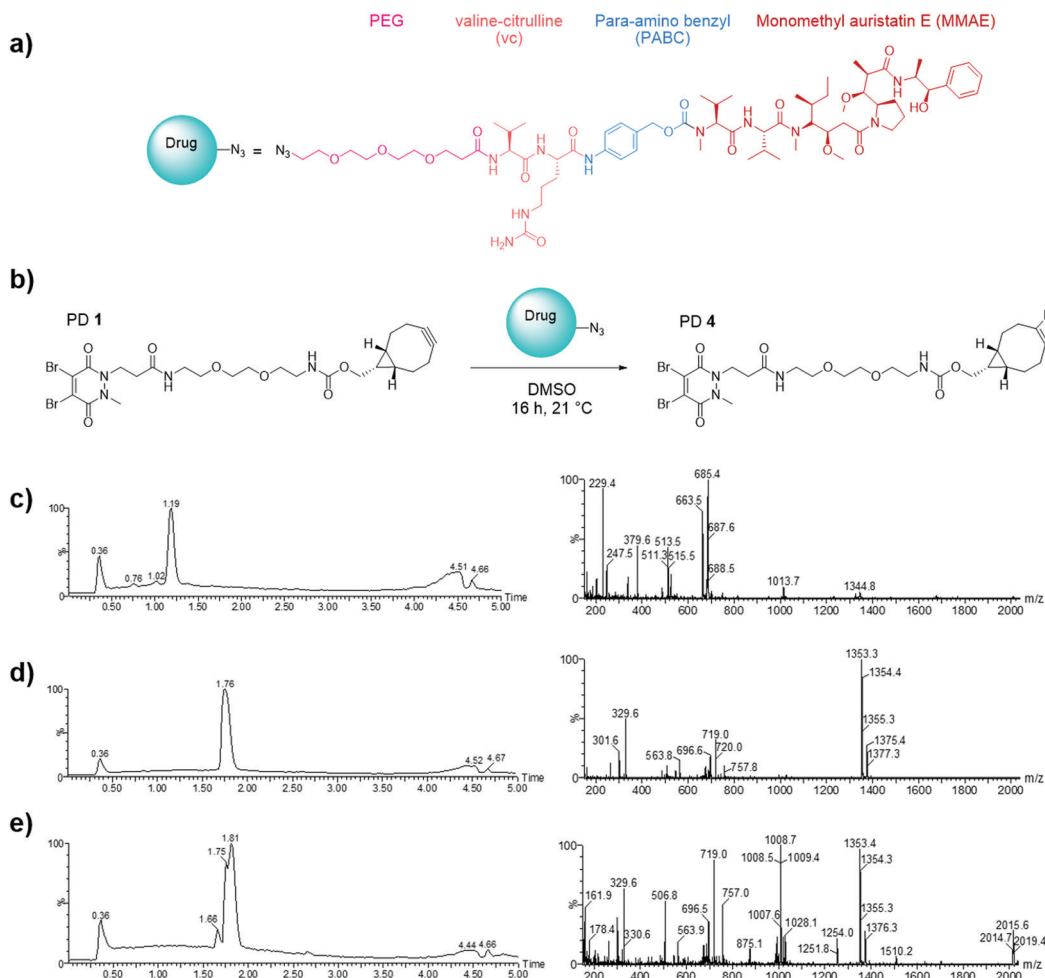
Fig. 6 Selection of drug for the generation of the hLRG1-targeting ADC. (a) Structure of \text{N}_3 -PEG 3 -vc-PABC-MMAE; (b) SPAAC 'click' functionalisation (the pre-click strategy) reaction between the strained alkyne bearing PD 1 and azide-linked MMAE to form PD 4. (c) LCMS analysis of PD 1 (662 Da); (d) \text{N}_3 -PEG 3 -vc-PABC-MMAE (1353 Da) and (e) pre-click reaction of PD 1 with \text{N}_3 -PEG 3 -vc-PABC-MMAE showing formation of PD 4 (2015 Da) and complete consumption of PD 1.
