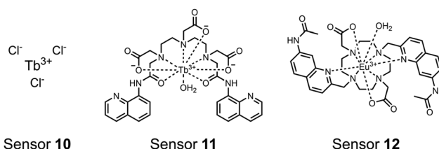
Fig. 4 Chemical structure of lanthanide chemosensors 10–12 .
