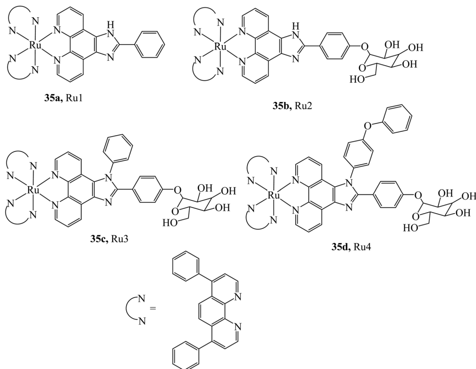
Fig. 17 [Ru(dpp)_2(pic-glucose)]^{2+} . 73
