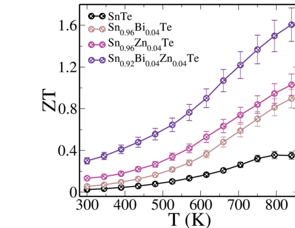
Fig. 5 ZT of SnTe and doped samples as a function of temperature. The ZT measurement uncertainty is about 10% (error bar).
