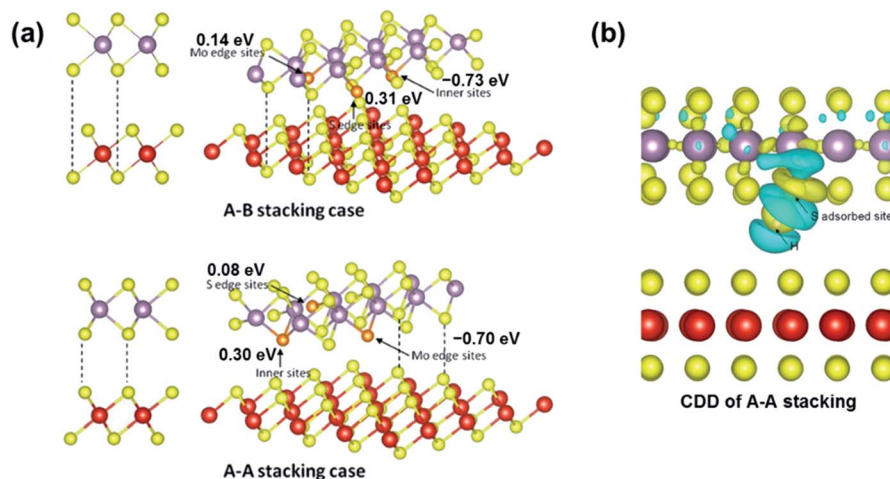
Fig. 12 (a) Two types of stacked bilayer structural models and their adsorption configurations. (b) CDD of the A-A stacking case (right) of the VS 2 @MoS 2 -edge nanosheet. The cyan and yellow regions represent the charge depletion and accumulation space, respectively. Reprinted with permission from ref. 35 Copyright 2017, ACS Publishing.
