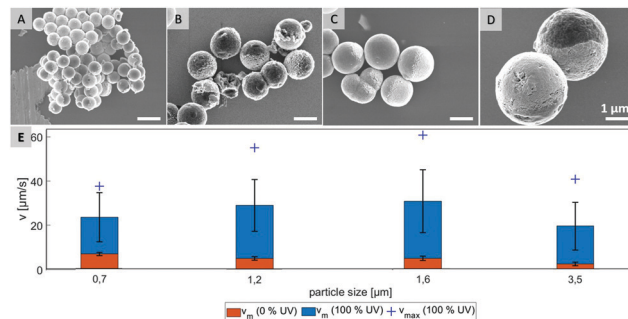
Fig. 3 SEM pictures of Janus particles with average sizes of 0.7 \mu\text{m} (A), 1.2 \mu\text{m} (B), 1.6 \mu\text{m} (C), 3.5 \mu\text{m} (D) and their velocities (E) in 0.5% \text{H}_2\text{O}_2 solution ( v_m – mean velocity at given UV intensity, v_{max} – velocity of fastest particle), scale bar 1 \mu\text{m} .
