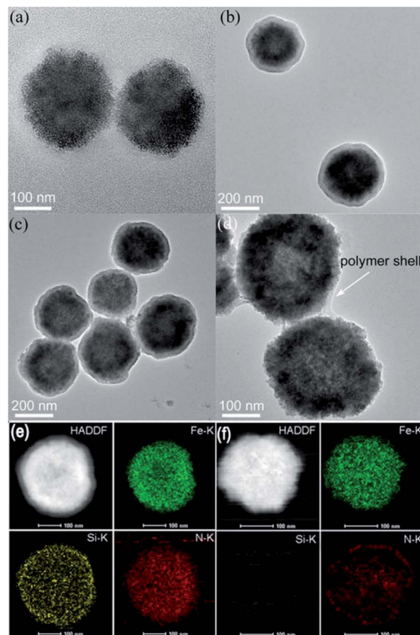
Fig. 1 TEM images of (a) \text{Fe}_3\text{O}_4 NPs, (b) \text{Fe}_3\text{O}_4@\text{SiO}_2 , (c) \text{Fe}_3\text{O}_4@\text{SiO}_2@\text{Poly(L-Trp)} , and (d) yolk-shell \text{Fe}_3\text{O}_4@\text{Poly(L-Trp)} . (e) and (f) show the TEM elemental mapping images of \text{Fe}_3\text{O}_4@\text{SiO}_2@\text{Poly(L-Trp)} and yolk-shell \text{Fe}_3\text{O}_4@\text{Poly(L-Trp)} , respectively.
