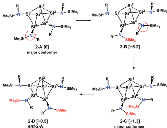
Scheme 5 Major and minor conformer and enantiomer of 2 in solution. Values in brackets are solvent corrected relative free energies ΔG(298) soln .
