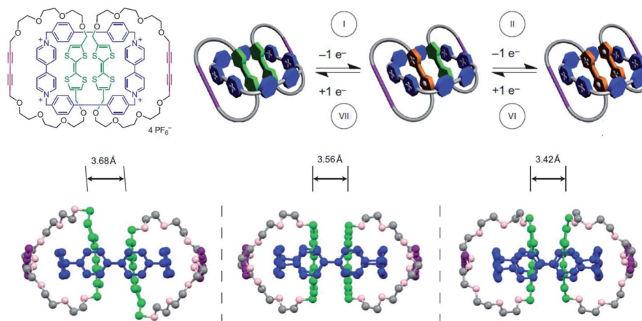
Fig. 17 The chemical structure of the [3]catenanes and their stepwise oxidation. The single crystal structure of (TTF) 2 , (TTF) 2 •+ and (TTF) 2 •• containing [3]catenanes. Reproduced from ref. 80 with permission from Nature Publishing Group, Copyright 2010.
