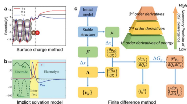
Scheme 1 The computational method for EC-IR and EC-Raman spectra: (a) surface charged method, (b) implicit solvation model and (c) finite difference method. \mu , F , X , A , \nu_k and G_Z represent the surface dipole moment, atomic force, external atomic coordinates, dynamical matrix at the T point, vibrational frequency of the k^{\text{th}} normal-mode coordinate Q_k , and external electric field along the Z axis, respectively. \Delta x and \Delta G_Z represent the step size of X and G_Z for the finite difference. Image (a) adapted from ref. 38 with permission, copyright (2011) Royal Society of Chemistry; image (b) adapted from ref. 29 with permission, copyright (2014) American Institute of Physics.
