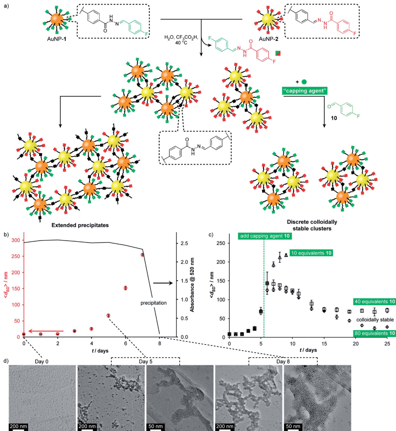
Fig. 6 (a) Assembly of complementary nucleophilic (AuNP-1) and electrophilic (AuNP-2) dynamic covalent nanoparticles to produce extended networks (b and d) or discrete colloidally stable clusters (c). (b) Average hydrodynamic diameter ( \langle d_{SD} \rangle ) for complementary assembly, as measured by DLS, and absorbance at 520 nm over time. (c) Average hydrodynamic diameter ( \langle d_{SD} \rangle ), as measured by DLS, showing the effect of introducing different concentrations of monofunctional capping agent 10 at day 5. (d) Representative TEM images at 0, 5 and 8 days. Conditions (all experiments): 0.15 mM overall surface-bound hydrazones, 9 : 1 v/v DMF/ \text{H}_2\text{O} , 20 mM \text{CF}_3\text{CO}_2\text{H} , 40^\circ\text{C} . Full UV-Vis absorption spectra, an expansion of solvodynamic sizes observed over days 1–4, and additional TEM images are reported in the ESI.†
