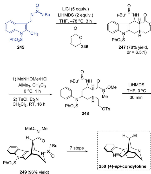
Scheme 41 Total synthesis of (+)- epi -condyfoline.
