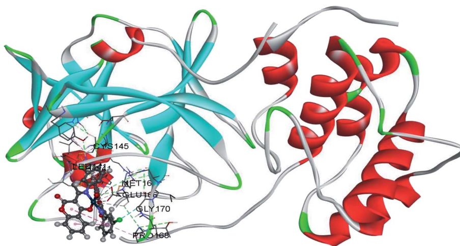
Fig. 5 The docking interactions of the most stable conformation of ligand (Pd(II) complex) with M pro of SARS-CoV-2.
