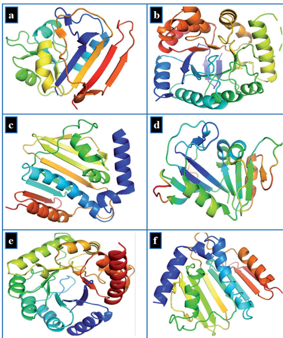
Fig. 3 3D-structure of target proteins of E. coli , (a) dihydrofolate reductase (PDB: 2ANQ), (b) dihydropteroate synthase (PDB: 5U0V), (c) DNA gyrase (PDB: 6KZX) and for S. aureus (d) dihydrofolate reductase (PDB: 3FY8), (e) dihydropteroate synthase (PDB: 4HB7), (f) DNA gyrase (PDB: 5CTU).
