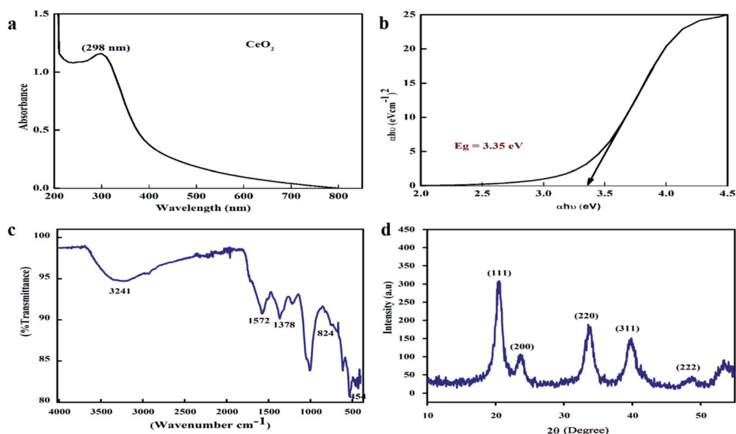
Fig. 2 (a) UV-visible spectrum, (b) Tauc plot, (c) FTIR spectra, and (d) XRD pattern of the biosynthesized \text{CeO}_2 -NPs.
