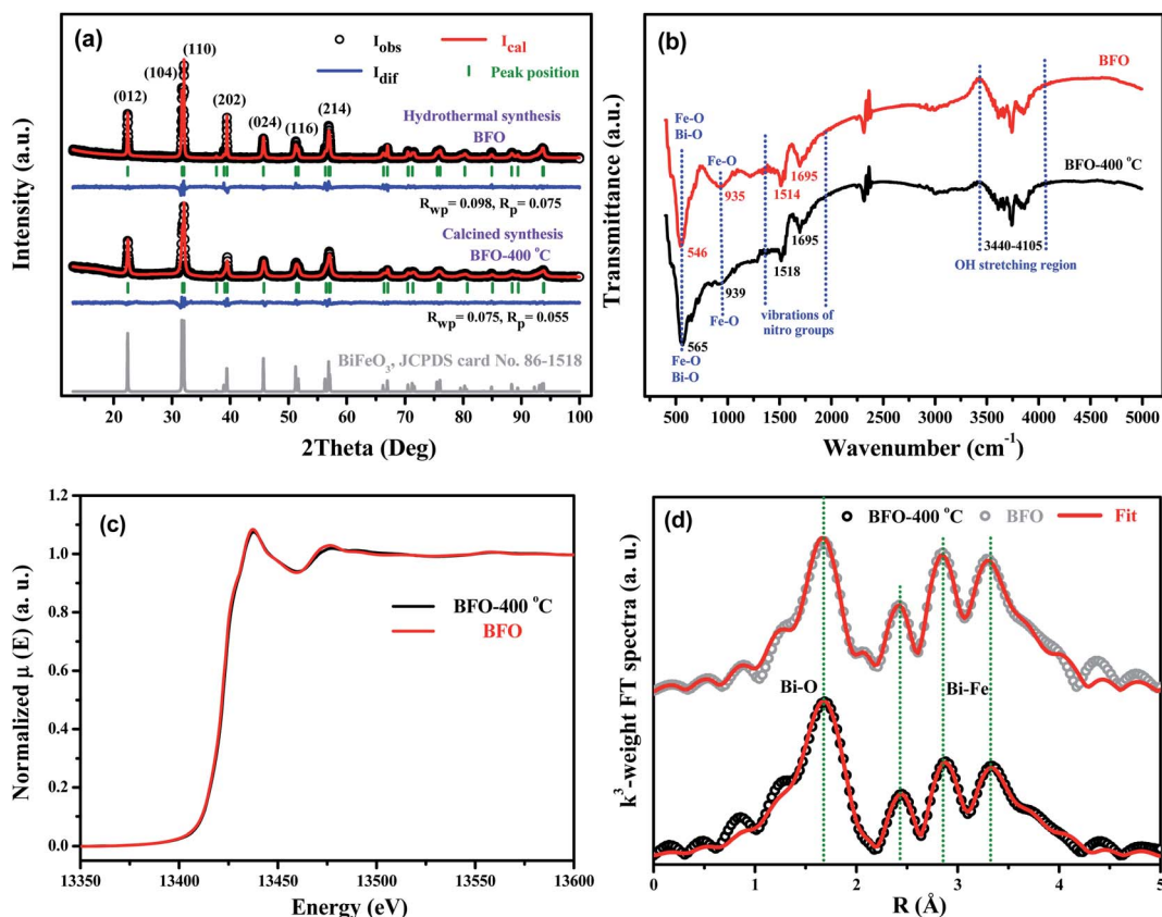
Fig. 10 (a) XRD patterns, (b) FTIR spectra, (c) \text{Bi L}_{3\text{-edge}} XAFS spectra and (d) FT spectra of EXAFS oscillations k^3\chi(k) for BFO-400 °C and BFO.
