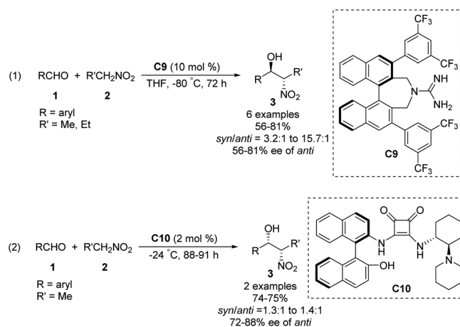
Scheme 31 Axially chiral guanidine catalysed Henry reactions.
