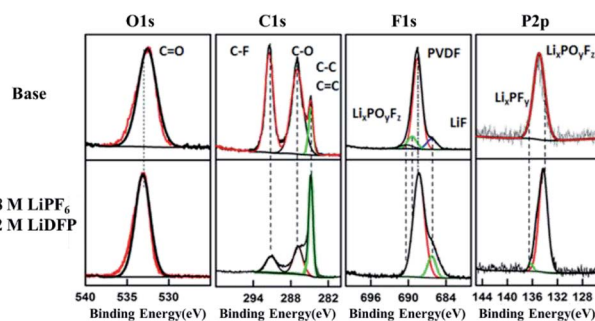
Fig. 6 C1s, O1s, F1s, P2p XPS spectra of cathode surface in base and dual-lithium salts electrolytes.
