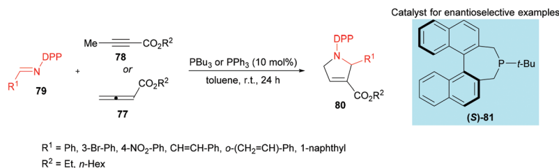
Scheme 18 Phosphine-catalyzed synthesis of pyrrolines from N -DPP-imines and allenolates/2-butynoates.
