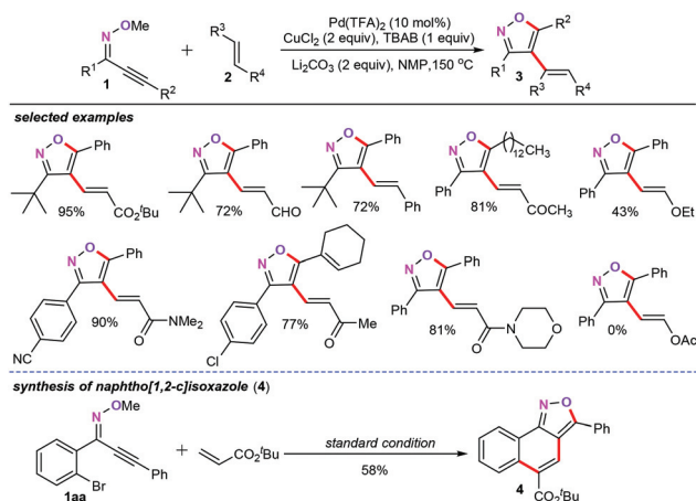
Scheme 1 Palladium-catalyzed cascade cyclization/alkenylation for the synthesis of trisubstituted isoxazoles.
