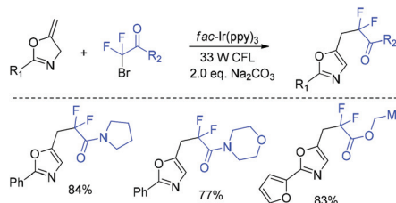
Scheme 32 The difluoroalkylation of alkenes.
