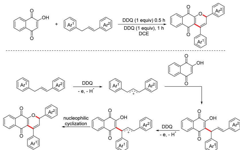
Scheme 46
