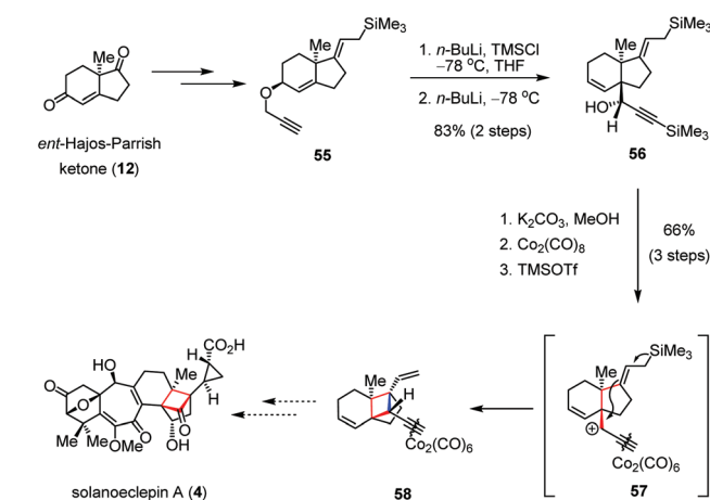
Scheme 8 Cationic Hosomi–Sakurai type cyclization towards the total synthesis of solanoeclepin A.
