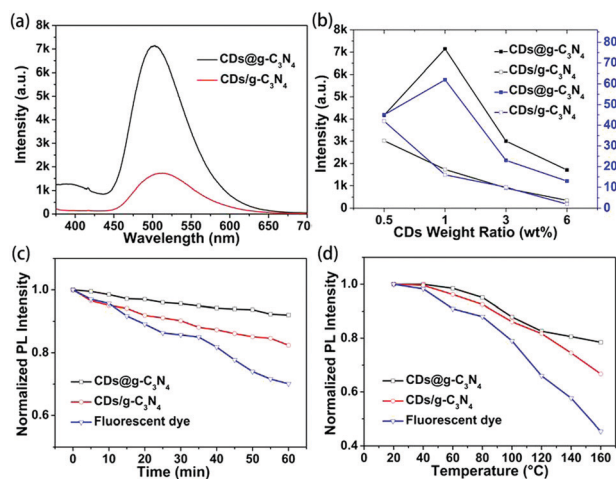
Fig. 5 (a) PL spectra of CD@-g-C 3 N 4 and CD@-g-C 3 N 4 composites with 1 wt% CD loading concentration under 360 nm excitation. (b) Peak PL intensities under 360 nm excitation of CD@-g-C 3 N 4 and CD@-g-C 3 N 4 with different CD loading concentrations (black curves) and PLQYs of CD@-g-C 3 N 4 and CD@-g-C 3 N 4 composites with different CD loading concentrations under 410 nm excitation (blue curves). Evolution of the PL intensities of CD@-g-C 3 N 4 , CD@-g-C 3 N 4 and organic dye (fluorescein sodium): (c) under UV light exposure (1.6 W cm -1 ) and (d) upon heating to 160 °C.
