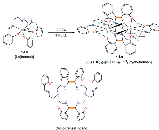
Scheme 4 Synthesis of [K(THF) 3 ] 2 (K(THF) 2 ) 2 Ln 2 (cyclo-trenal), 4-Ln , Ln = Nd, Sm.
