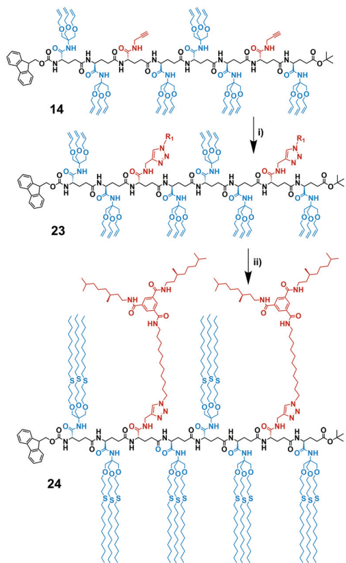
Scheme 6 Synthesis of bis((S)-BTA)-hexa(tris(decylaloyloxy))Fmoc-(TTAT 2 )-COOtBu ( 24 ). Reagents and conditions: (i) (1) BTA-azide 20 , CuSO 4 , sodium ascorbate, DMSO, 50 °C → room temperature, argon atmosphere, overnight at room temperature; (2) CuSO 4 , sodium ascorbate, DMSO, 50 °C → RT, argon flow, 2 days at room temperature, 37%; (ii) 1-decanethiol, DMPA, DMA, hν, argon, 4 h at room temperature, 31%.
