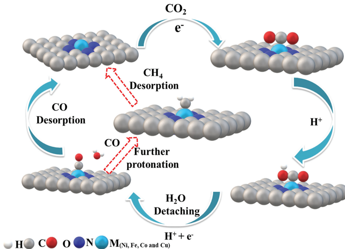
Fig. 7 Proposed reaction paths for CO 2 electroreduction by M–N–C. Fe–N–C follows the red arrow to further undergo protonation to give methane (CH 4 ).
