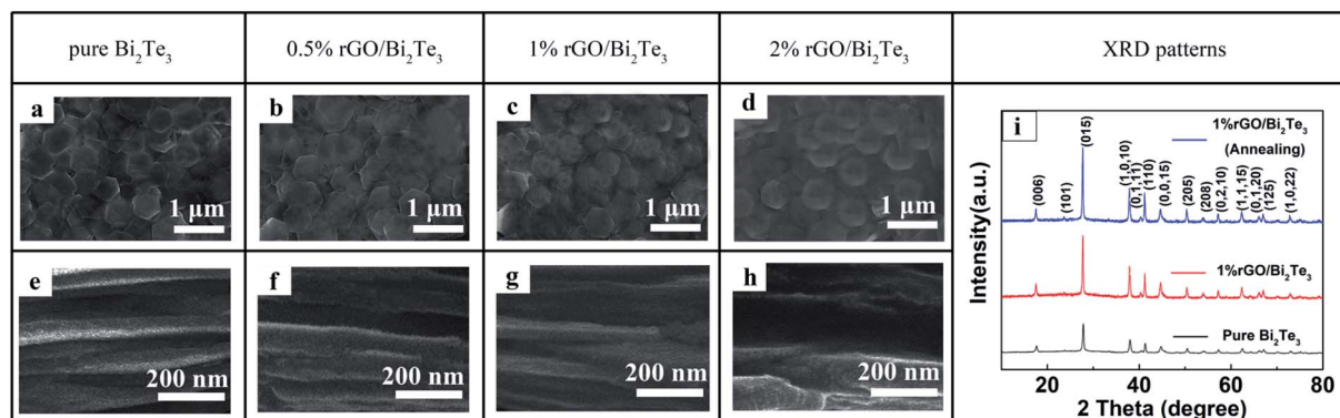
Fig. 1 Surface and cross-sectional SEM images of \text{Bi}_2\text{Te}_3 nanoplale films with different mass ratio of rGO nanosheets: (a) and (e) pure \text{Bi}_2\text{Te}_3 , (b) and (f) 0.5% \text{rGO}/\text{Bi}_2\text{Te}_3 , (c) and (g) 1% \text{rGO}/\text{Bi}_2\text{Te}_3 , and (d) and (h) 2% \text{rGO}/\text{Bi}_2\text{Te}_3 ; (i) XRD patterns of the pure \text{Bi}_2\text{Te}_3 and 1% \text{rGO}/\text{Bi}_2\text{Te}_3 composites films before and after annealing.
