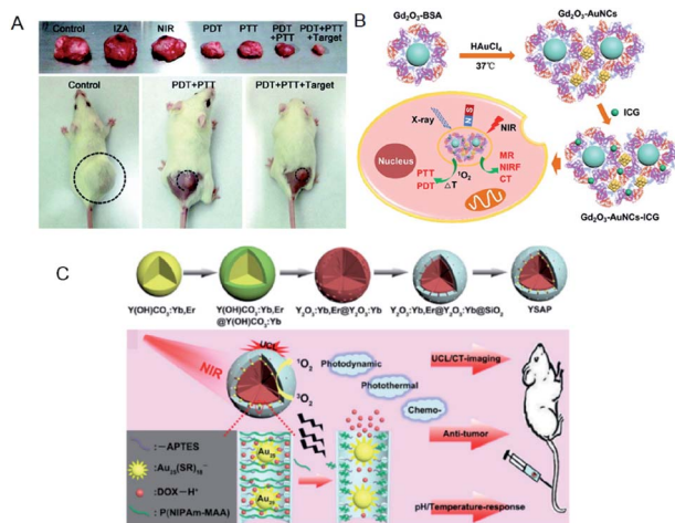
Fig. 22 (A) Photographs of tumor tissues excised from mice on the 14th day of treatment using normal saline, pure NIR laser, IZA:MOFs of Fe 3 O 4 /ZIF-8-Au 25 , PDT (pure Au 25 (Capt) 18 NCs under NIR), PTT (IZA under NIR), PDT + PTT, and PDT + PTT + magnetic stimulus. Bottom: photographs of representative tumor-bearing mice on the 14th day. (B) Schematic of Gd 2 O 3 -AuNCs-ICG nanohybrid as theragnostic agent for imaging-guided cancer therapy. (C) Schematic for the formation of Y 2 O 3 :Yb,Er@Y 2 O 3 :Yb@mSiO 2 -Au 25 P(NIPAm-MAA) and the imaging-guided synergistic multimodal anti-cancer therapy. Panel (a) is reproduced with permission from ref. 127. Copyright 2015 Royal Society of Chemistry. Panel (b) is reproduced with permission from ref. 134. Copyright 2017 American Chemical Society. Panel (c) is reproduced with permission from ref. 129. Copyright 2015 Elsevier Ltd.
