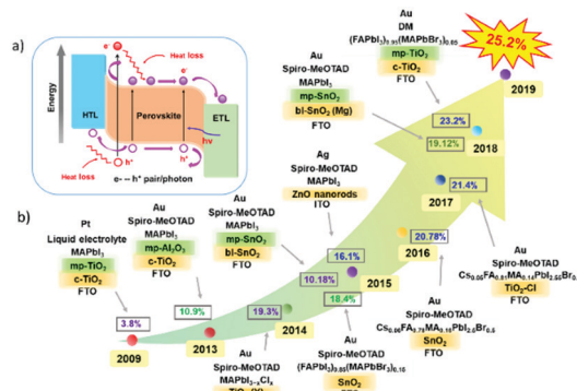
Fig. 3 (a) Schematic diagram and energy band of interfaces among the electron transport layer (ETL)/perovskite/hole transport layer (HTL). (b) The representative progress of ETLs in the n - i - p architecture.
