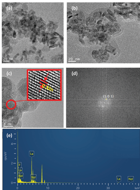
Fig. 3 HRTEM images of (a) \text{Nd}^{3+} - \text{LaF}_3 -0.04 M powder and (b) \text{Nd}^{3+} - \text{LaF}_3 -PVP(10)-0.25 M powder (c) single nanocrystal showing a lattice spacing of 0.32 nm for sample 0.9\text{Nd}^{3+} - \text{LaF}_3 -0.25 M-PVP(10) (d) FFT pattern corresponding to (c) and (e) EDX analysis of the region.
