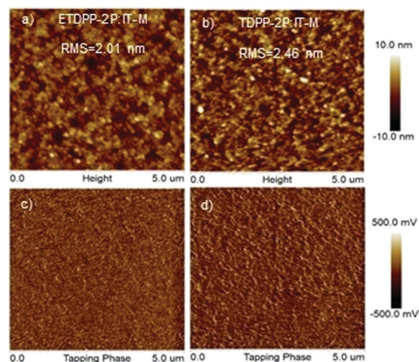
Fig. 5 AFM height images (a and b) and phase images (c and d) of the binary blend films ETDPP-2P/IT-M and TDPP-2P/IT-M from left to right. The scan size is 5 \mu m \times 5 \mu m for all images.
