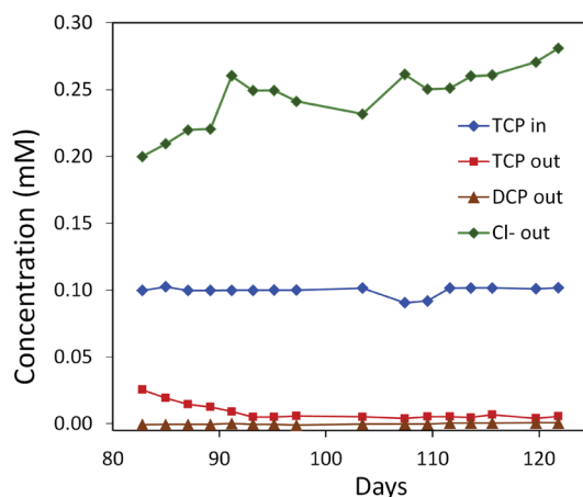
Fig. 6 Degradation of TCP by a mixed culture of P. putida strains MC4-5221, MC4-5222, MC4-1331 and A. radiobacter AD1 in a laboratory-scale aerated packed bed bioreactor operated in a continuous mode. Packing material was sintered glass and data were collected after an initial 80 day acclimation period. TCP loading rate 0.40–0.44 mg h -1 l -1 ; residence time 23 h; removal increasing to 95%. 40,62
