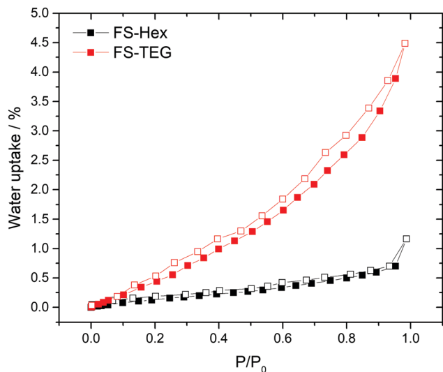
Fig. 3 Water vapor isotherms of FS-Hex and FS-TEG at 20.0 \text{ }^\circ\text{C} and up to 23 \text{ mbar} .
