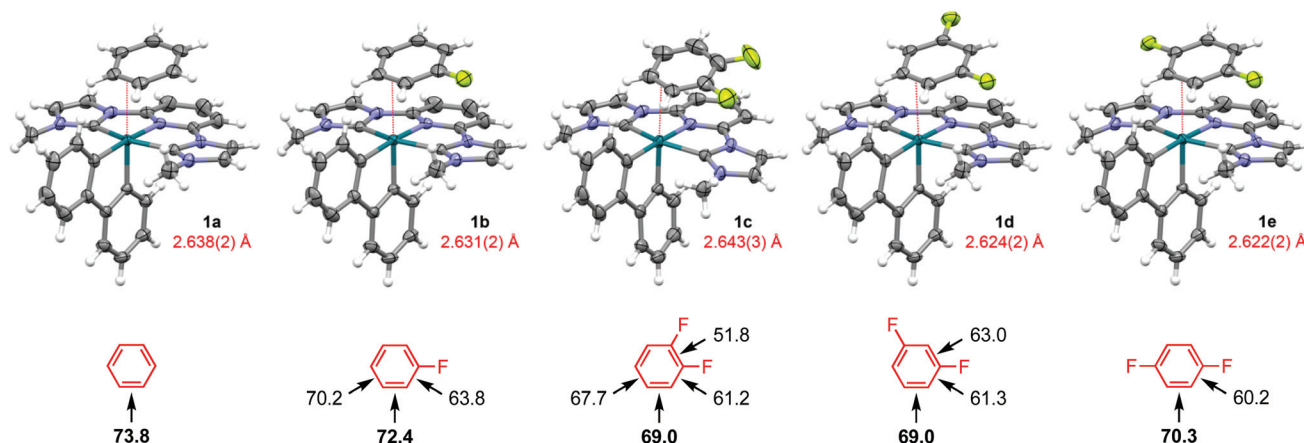
Fig. 1 Solid-state structures of \eta^2 -arene complexes 1a–e (top) and calculated binding energies (kJ mol −1 , bottom). Solid-state structures drawn with thermal ellipsoids at 50% probability, minor disordered components (local symmetry equivalent F atom in 1b ) and [B(3,5-(CF 3 ) 2 C 6 H 3 ) 4 ] − anion omitted for clarity.
