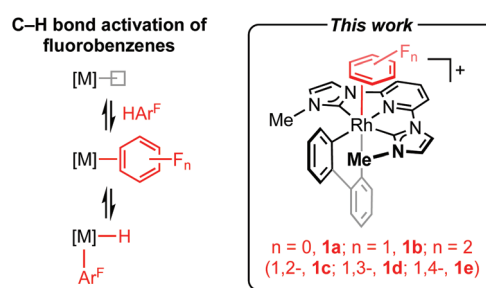
Scheme 1 Intermediacy of \eta^2 -adducts in the C–H bond activation of fluoroarenes. [B(3,5-(CF 3 ) 2 C 6 H 3 ) 4 ] − anion omitted for clarity.
