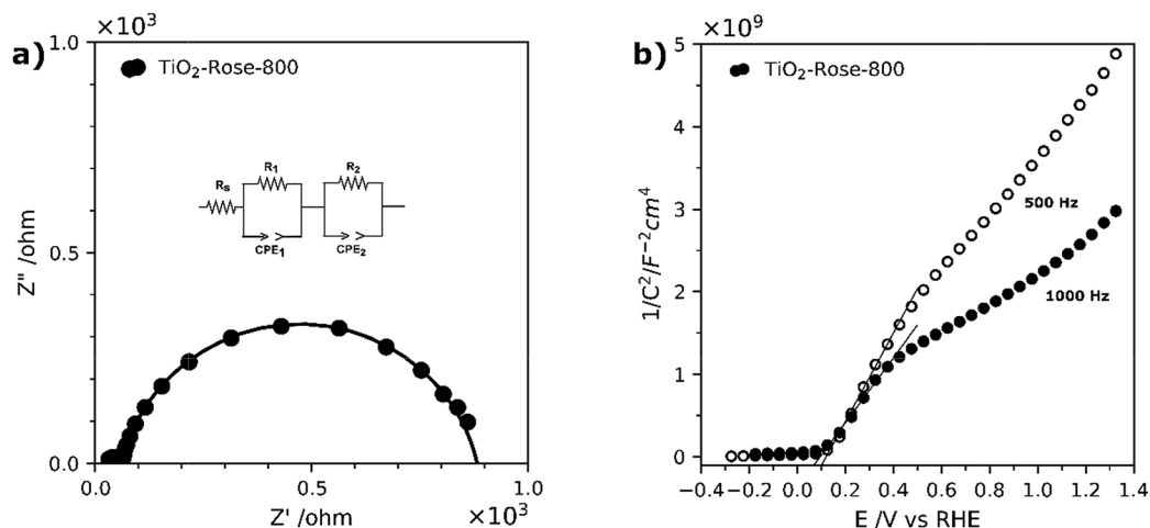
Fig. 10 (a) Nyquist plots of \text{TiO}_2 -Rose-800 at the open circuit potential (OCP) of the cell under 1 sun illumination ( \text{AM } 1.5\text{G} , 100 \text{ mW cm}^{-2} ). (b) Mott-Schottky plots at a fixed frequency of 500 Hz and 1000 Hz of \text{TiO}_2 -Rose-800 in 1 M KOH ( \text{pH} = 13.6 ).
