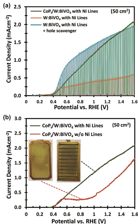
Fig. 5 (a) J - V curves under constant, dark and chopped AM 1.5G illumination comparing the performance of large area ( 50 \text{ cm}^2 ) \text{W}:\text{BiVO}_4 photoanodes with Ni lines, either in 2.0 M \text{KP}_i buffer solution with 0.5 M \text{Na}_2\text{SO}_3 (blue), or without hole scavenger, before (orange) and after (green) photo-electrodeposition of \text{CoP}_i . (b) J - V curves comparing \text{CoP}_i -modified \text{W}:\text{BiVO}_4 photoanodes with (green) and without (red) Ni lines measured in 2.0 M \text{KP}_i buffer, pH 7, under AM 1.5G illumination. Inset: photographs of the \text{CoP}_i deposited on \text{W}:\text{BiVO}_4 photoanodes without (left) and with (right) Ni lines.
