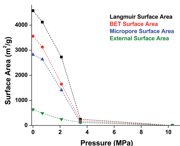
Fig. 5 Surface area of MOF-5 as a function of pressure. Elevated pressures were obtained using an anvil press in the absence of pressure transmitting fluid. Surface area values were determined using \text{N}_2 adsorption measurements at 77 K. Adapted with permission from ref. 47. Copyright 2010 by American Physical Society.
