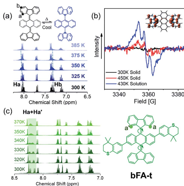
Fig. 4 (a) VT- 1 H NMR of bFA in tetrachloroethane- d 2 ; (b) EPR data of bFA in the solid state at 300 K (black) and 450 K (red) and in dichlorobenzene (4 × 10 -2 M) at 430 K (blue); inset: spin density illustration of the T_1 state of bFA twist (twisted configuration) at the UMO6L/6-311G** level of theory; (c) VT- 1 H NMR of bFA-t and the molecular structure of bFA-t .
