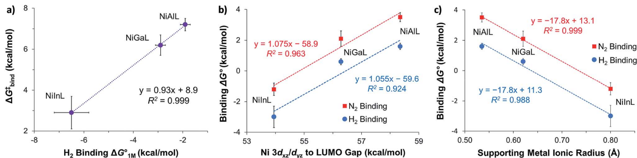
Fig. 7 (a) Plot of free energy barrier for \text{H}_2 binding ( \Delta G_{\text{bind}}^\ddagger ) vs. thermodynamic free energy for \text{H}_2 binding ( \Delta G_{1\text{M}}^\circ ), with the standard deviation in all values shown by error bars and all standard states defined to be [\text{H}_2] = 1 \text{ M} in toluene- d_8 . (b–c) Plots of \Delta G^\circ for \text{H}_2 (blue circles) and \text{N}_2 binding (red squares) vs. Ni 3d xz /d yz to LUMO energy gap (b) and vs. supporting metal Shannon ionic radii (c). Ni 3d xz /d yz to LUMO energy gaps were measured experimentally by UV-Vis spectroscopy with transition assignments from TD-DFT calculations (see ESI† and Table 5).
