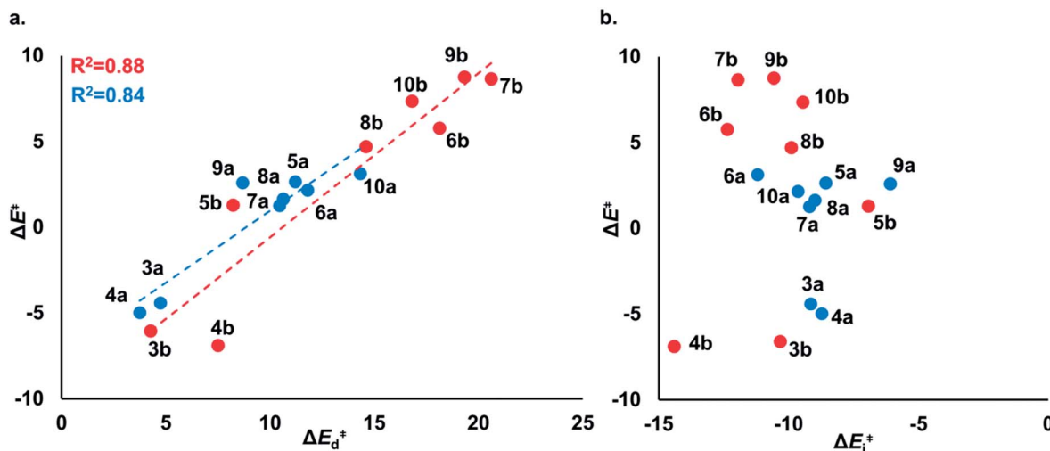
Fig. 4 (a) \Delta E^\ddagger vs. \Delta E_d^\ddagger of the nucleophilic addition of \text{MeS}^- towards cyclic thiosulfates (blue) and cyclic disulfides (red). The linear equation for (3–10)a is \Delta E^\ddagger = 0.84\Delta E_d^\ddagger - 7.40 . The linear equation for (3–10)b is \Delta E^\ddagger = 0.96\Delta E_d^\ddagger - 10.12 . (b) \Delta E^\ddagger vs. \Delta E_i^\ddagger of the nucleophilic addition of \text{MeS}^- towards cyclic thiosulfates (blue, R^2 = 0.001 ) and cyclic disulfides (red, R^2 = 0.05 ). Computed using M06-2X/6-311+G(d,p) IEF-PCM H 2 O . The energies are reported in \text{kcal mol}^{-1} .
