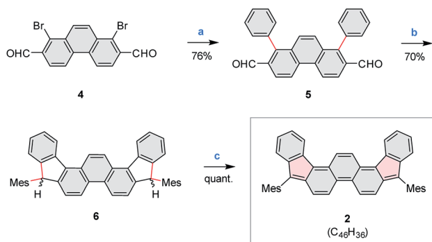
Scheme 2 Synthesis of 5,10-dimesityldiindeno[1,2- a :2',1'- i ]phenanthrene ( 2 ). Reagents and conditions: (a) PhB(OH) 2 , Pd(PPh 3 ) 4 , Na 2 CO 3 (aq), dioxane, reflux, overnight. (b) (1) MesMgBr, THF, rt, overnight. (2) BF 3 ·Et 2 O, DCM, rt, 10 min. (c) 2.5 equiv. DDQ, toluene, rt, overnight.
