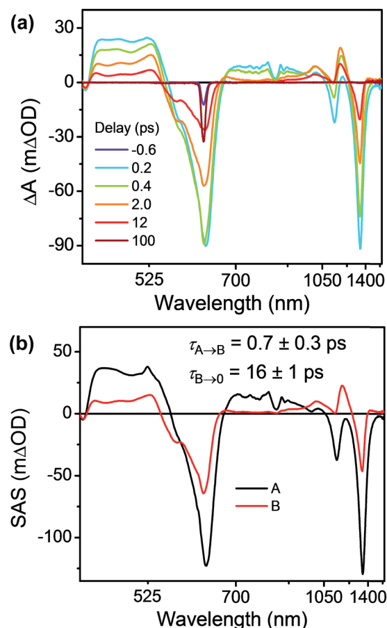
Fig. 8 (a) fsTA spectra and (b) species-associated spectra (SAS) of Per ⊂ TTzExVBox 3++ in CH 3 CN excited at 620 nm ((A) 2 *TTz 2+ (D n ), (B) TTz 2+ -Per-ExV 2+ ). The wavelength axis is plotted in reciprocal space. Time constants are for the representative data set shown here; averages and standard deviations from multiple experiments are given in Table 1.
