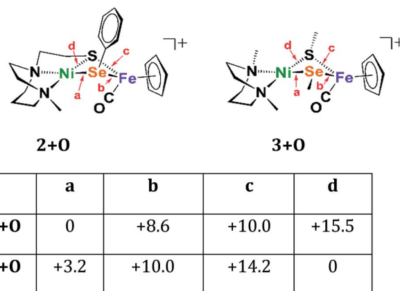
Fig. 6 Relative energies of oxygenated isomers of \text{N}_2\text{SSe}_{\text{Ph}} model, 2+O , and the bidentate, separated donors in the \text{N}_2\text{S}_{\text{Me}}\text{Se}_{\text{Me}} model, 3+O , in \text{kcal mol}^{-1} . A range of functionals and basis sets were explored and found to elicit minor differences on energies of complexes but do not change the ordering of isomers' energies (Fig. S41†).
