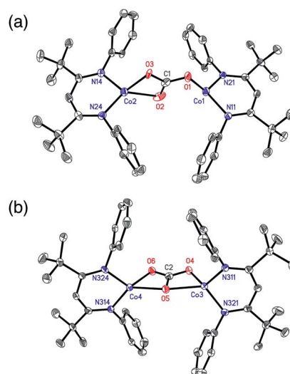
Fig. 1 The two crystallographically independent molecules in the crystal structure of 4: (a) μ-η 1 :η 2 form, with the major disorder component shown; (b) μ-η 2 :η 2 . H atoms and t Pr groups are omitted for clarity. Thermal ellipsoids are shown at 50% probability.
