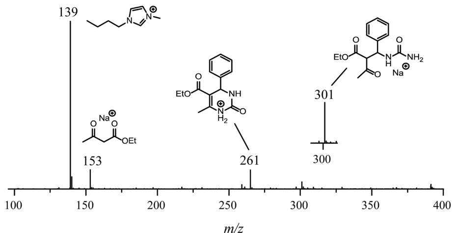
Fig. 7 ESI-MS(+) monitoring of the Biginelli reaction in the presence of the ionic liquid BMI·PF 6 after 5 min of reaction. Reaction conditions: catalyst (0.5 mol%), BMI·PF 6 (5.0 \mu M), benzaldehyde (5.0 \mu M), ethyl acetoacetate (5.0 \mu M), and urea (5.0 \mu M). The analyses were performed by dissolving the reaction mixture in methanol to afford the described concentrations. The inset is a 12-fold expansion to show the intermediate of m/z 301 prior to the final cyclization step affording the Biginelli adduct.
