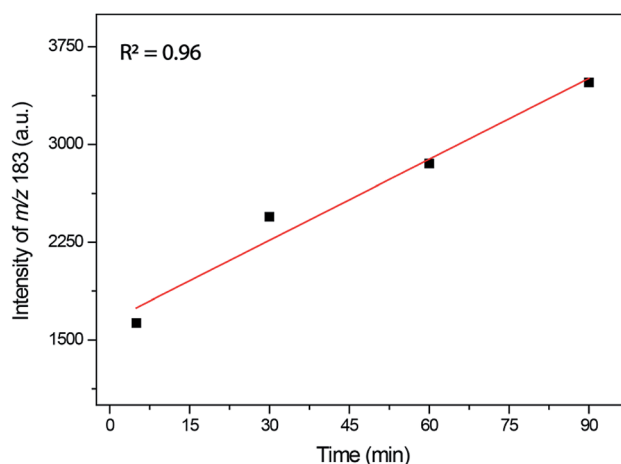
Fig. 8 Monitoring of the iminium intermediate ( m/z 183) by ESI(+)-MS during the reaction time. Reaction conditions: catalyst (0.5 mol%), BMI·PF 6 (5.0 \mu M), 4-chloro benzaldehyde (5.0 \mu M) instead of benzaldehyde, ethyl acetoacetate (5.0 \mu M), and urea (5.0 \mu M). The analyses were performed by dissolving the reaction mixture in methanol to afford the described concentrations.
