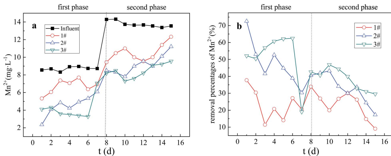
Fig. 7 (a) Mn 2+ residual concentration in Columns 1, 2, 3 (b) The removal percentage of Mn 2+ in Columns 1, 2, 3. Influent is the Mn 2+ concentration in influent water of AMD. 1#, 2# and 3# in (a) are the residual Mn 2+ concentration in AMD after repairing AMD with Column 1, Column 2 and Column 3 respectively. 1#, 2# and 3# in (b) are the removal percentage of Mn 2+ in AMD by the three dynamic columns corresponding to (a) respectively.
