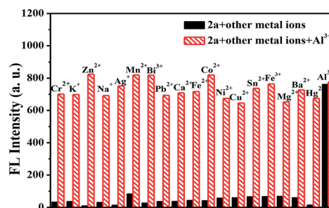
Fig. 2 Fluorescence intensity of 2a ( 5.0 \times 10^{-6} M) in buffer solution (EtOH/HEPES buffer, v/v = 6/4, 10 mM HEPES, pH = 7.4) and its complexes with \text{Al}^{3+} ( 5.0 \times 10^{-5} M) in the presence of various metal ions ( 5.0 \times 10^{-5} M), \lambda_{\text{ex}} = 330 nm.
