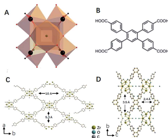
Fig. 1 Crystal structure of Zr-CAU-24 that is constructed from the [\text{Zr}_6(\mu_3\text{-O})_4(\mu_3\text{-OH})_4]^{12+} clusters (A) and \text{TCBP}^{4+} molecules (B). Ball-stick models of Zr-CAU-24 crystals (C) and (D).
