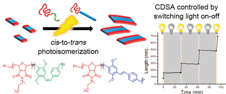
Fig. 8 Schematic illustration of the formation of nanofibers through the LI-CDSA of PNB- b -MeO-PPV) block copolymer. Reproduced with permission from ref. 60. Copyright 2018, American Chemical Society.
